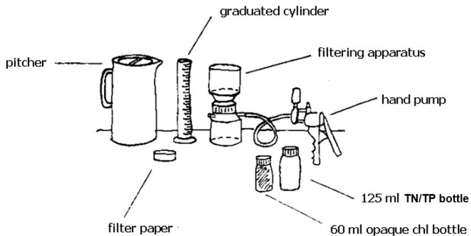
TN/TP and Chlorophyll a Sampling Gear
